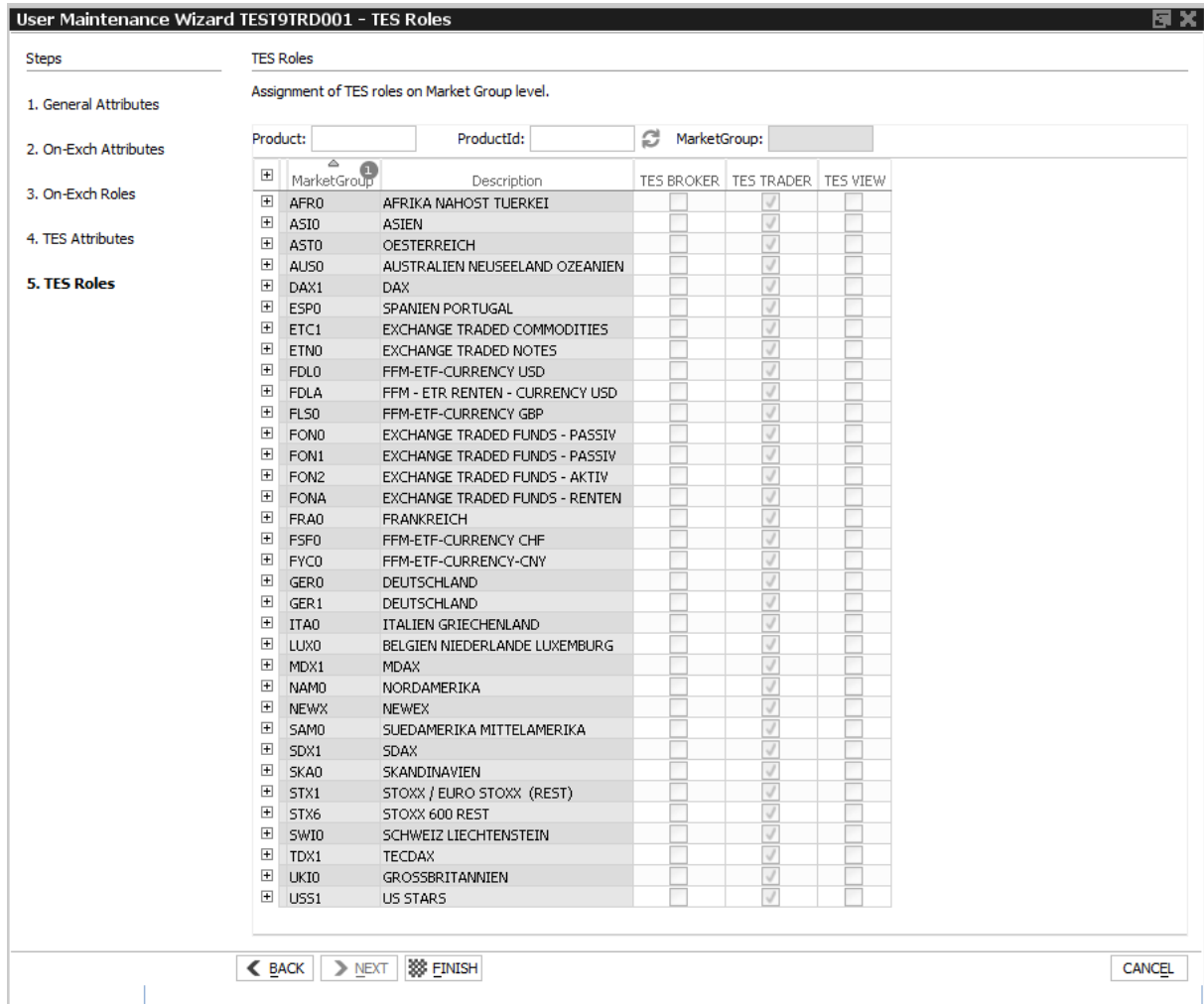
Image 10: T7 Admin GUI User Maintenance Wizard – TES Roles
