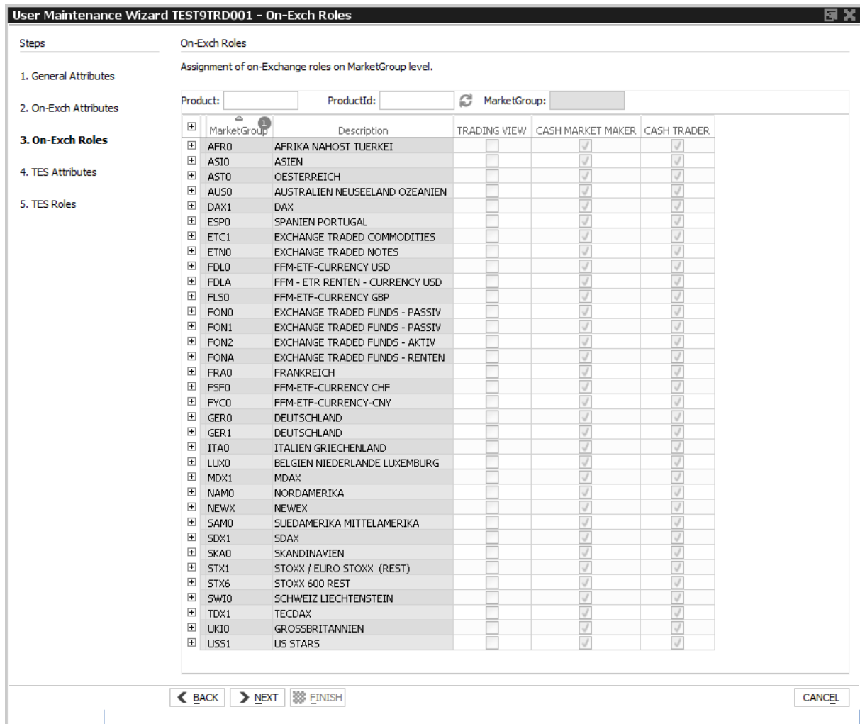
Image 8: T7 Admin GUI User Maintenance Wizard – On-Exch Roles
