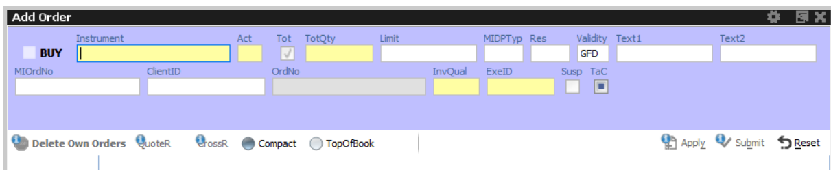
Fig. 55: Screenshot of the Order Entry view in compact mode and TopOfBook pane hidden
