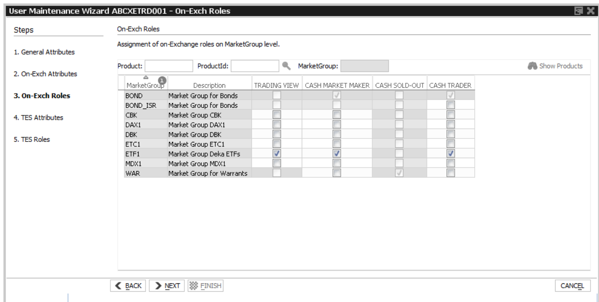
Fig. 97: Screenshot of the User Maintenance Wizard showing the entitlement roles on the On-Exch Roles tab
