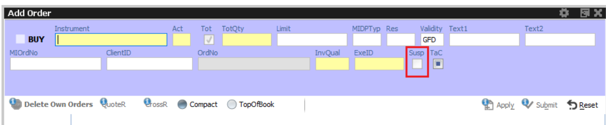
Fig. 59: Screenshot of the Order Entry showing the Susp checkbox
