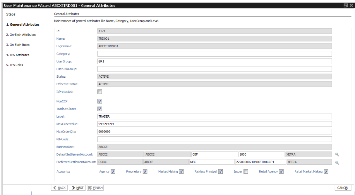
Fig. 98: Screenshot of the User Maintenance Wizard showing the General Attributes tab
