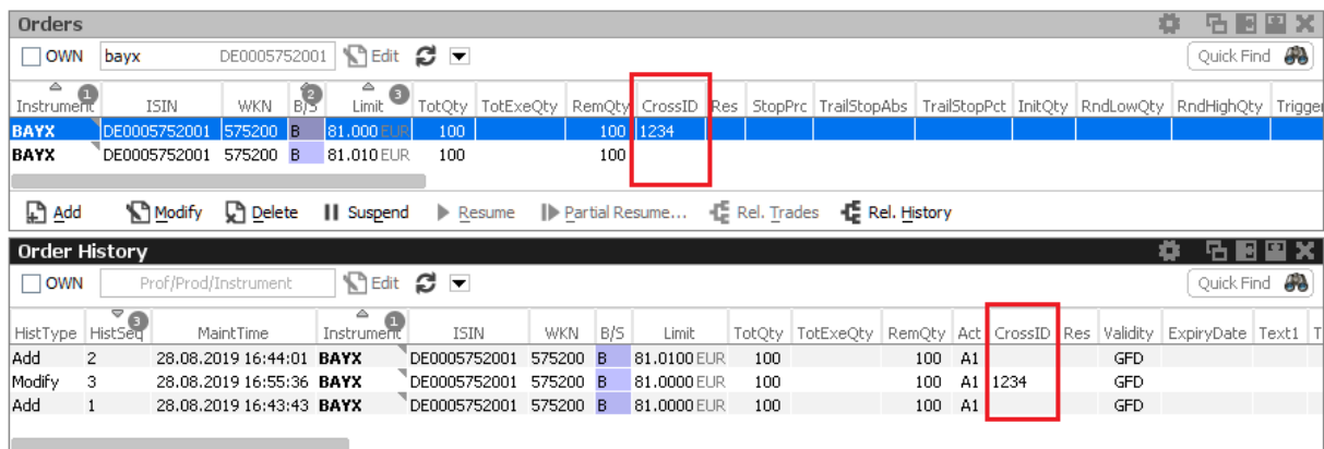
Fig. 62: Screenshots showing the CrossID column of the Orders and Order History view
