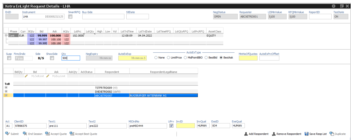
Fig. 75: Screenshot of the Xetra EnLight Request Details view depicting enabled AutoExType
