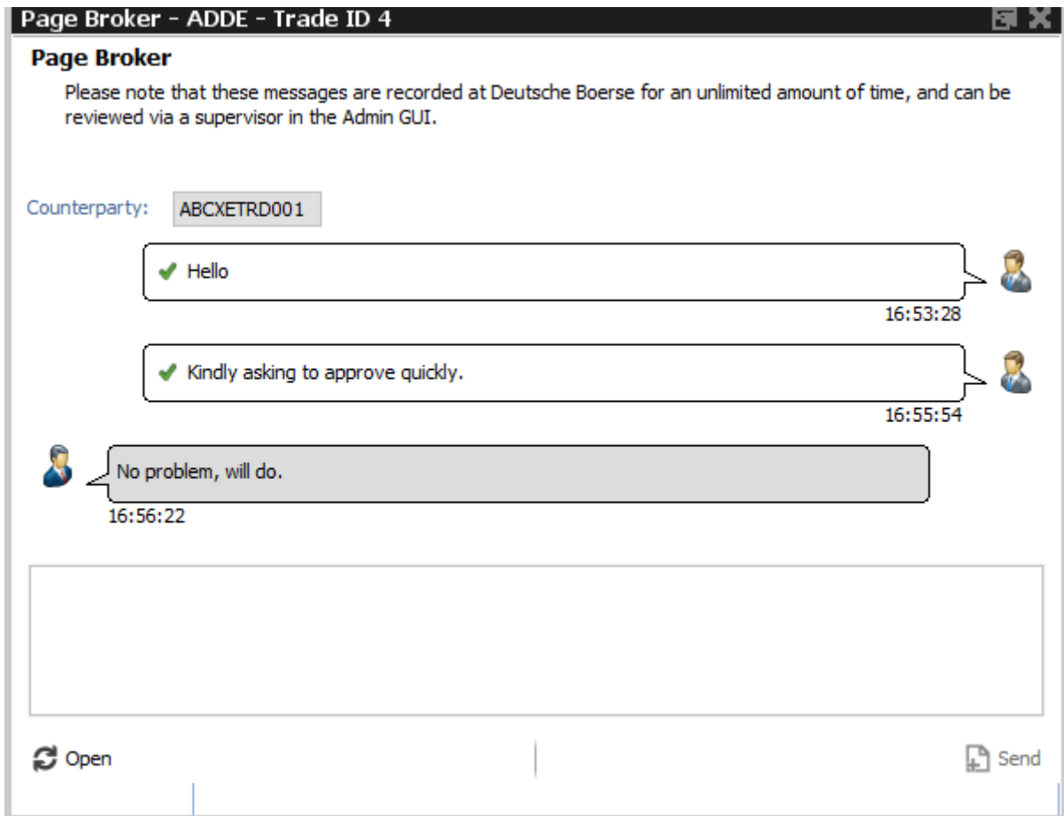
Fig. 69: Screenshot of the Page Broker dialogue
